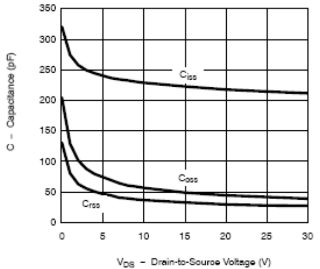
Capacitance
