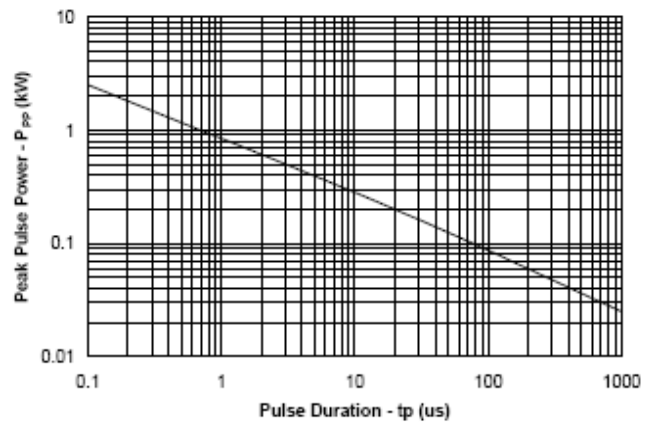
Fig 2 : Peak Plus Power V.S Exponential Pulse Duration
