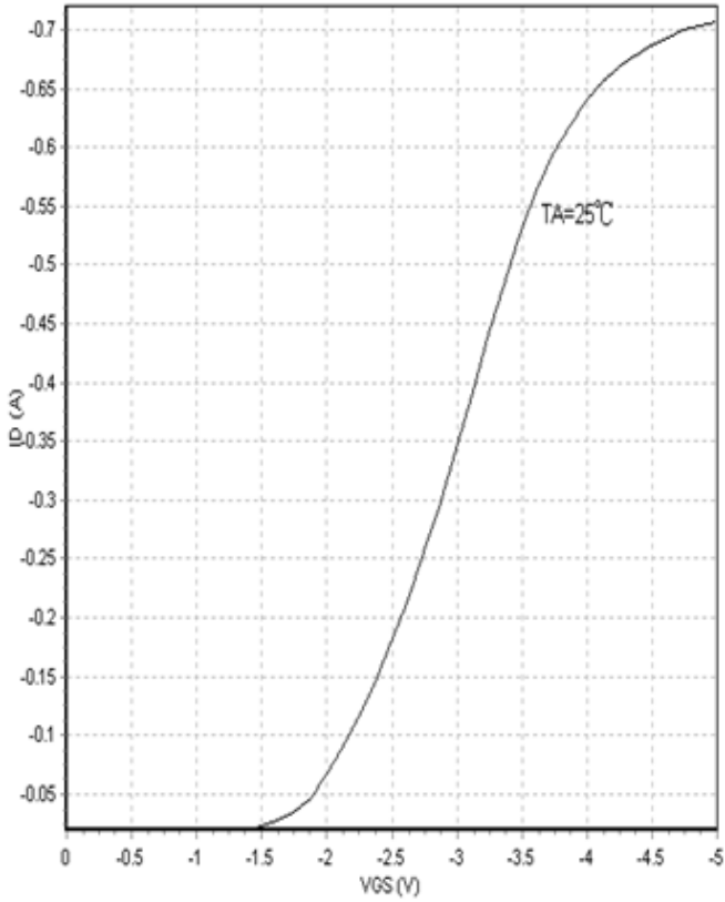
Drain-Current vs. Gate-Source Voltage
