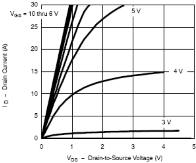
Output Characteristics
